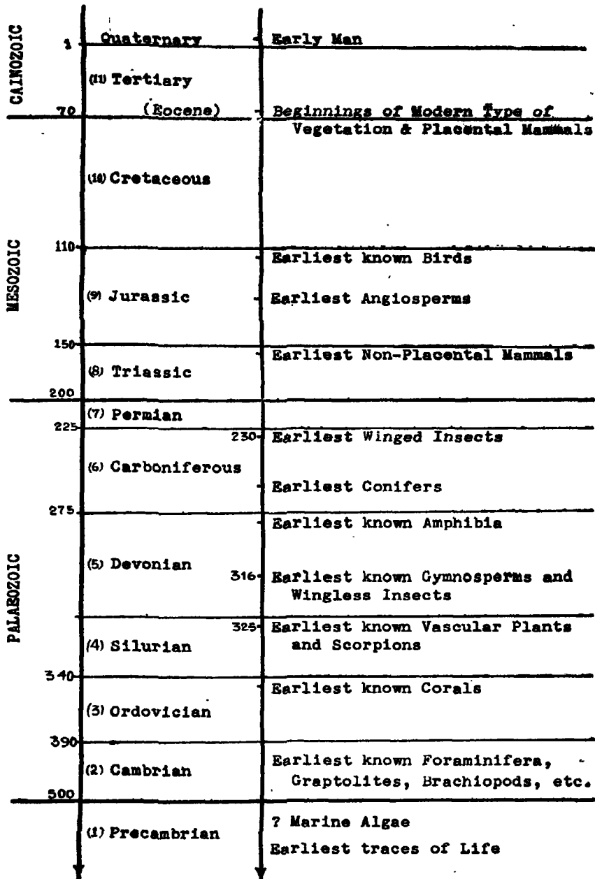
Fig. 4 - The Standard Stratigraphical Scale (simplified from Zeuner, "Dating the Past" 1946). The numbers without brackets represent the approximate ages of the strata in millions of years. Not drawn to scale.
